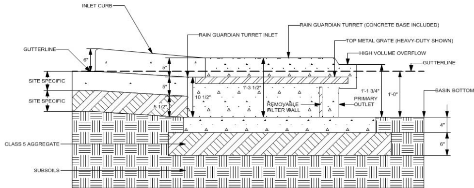
RAIN GUARDIAN TURRET CROSS-SECTION VIEW U.S. PATENT 8,501,016
